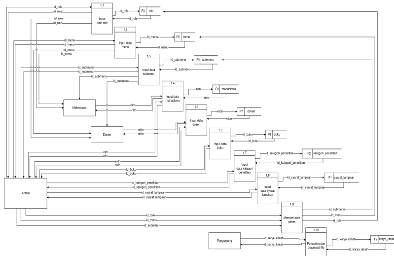
Gambar 6. Diagram Alir Data Level 1
