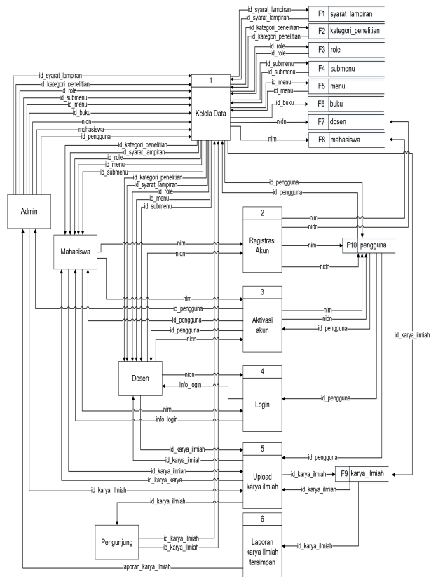
Gambar 5. Diagram Alir Data Level 1
